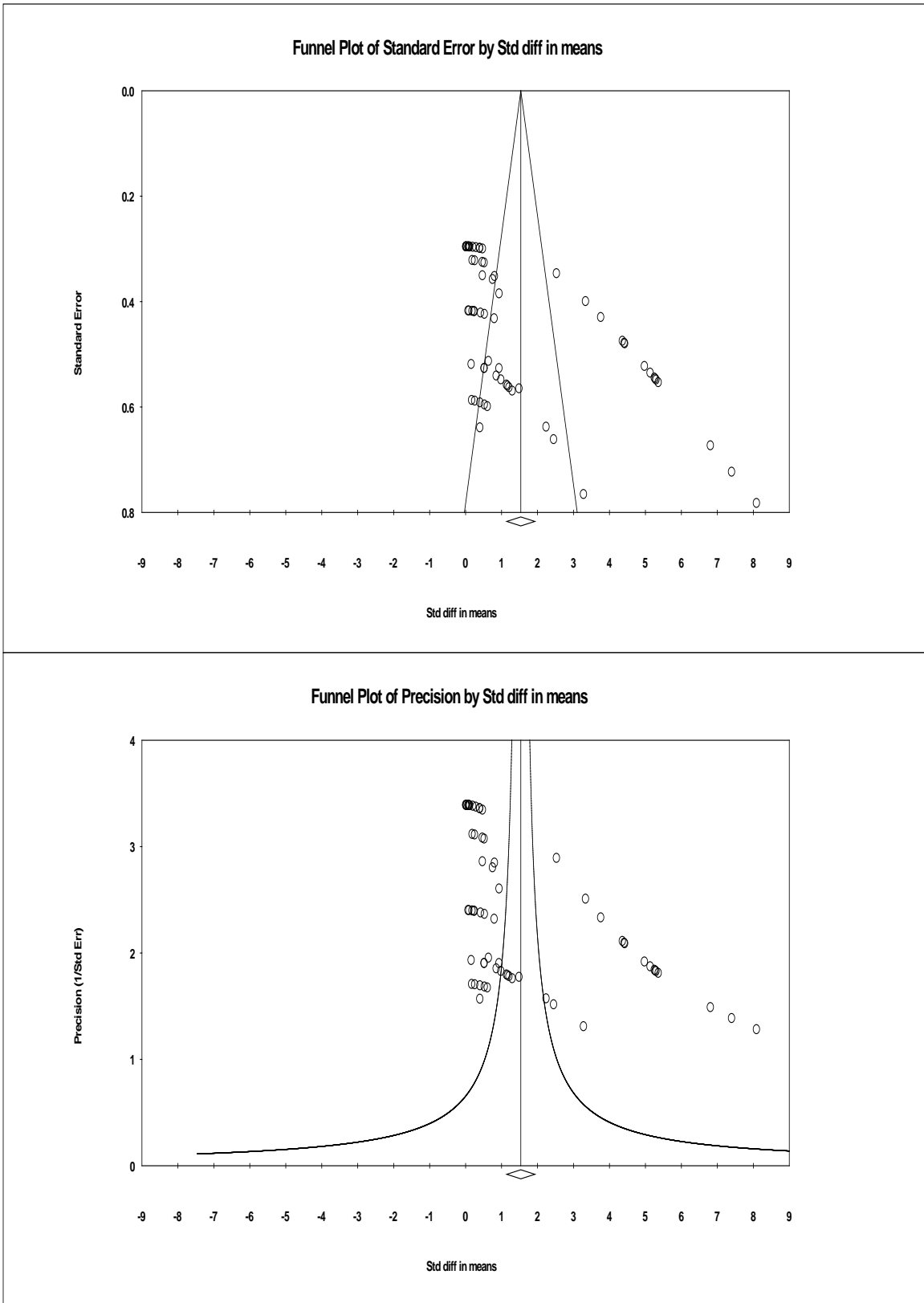
Figure 9. Funnel Plot of all 67 outcomes – random effect model
