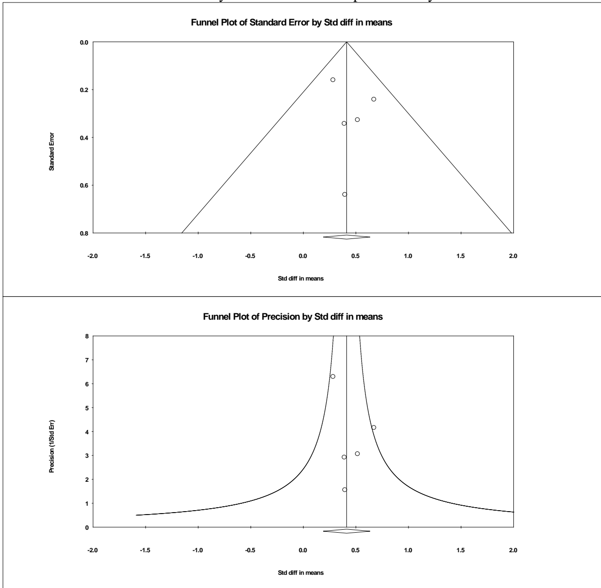
Figure 35. Funnel Plot of Physiological & Biometric Indicator (adjusted PHY) – fixed effect model
