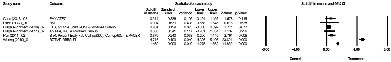
Figure 18. Forest Plot of Physiological & Biometric Indicator (PHY) – fixed effect model *only the first author and publication year were shown
